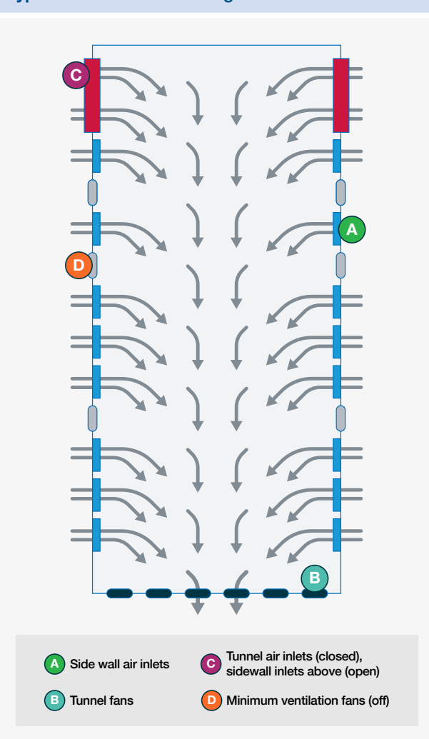
Figure 106 Typical air movement during transitional ventilation.
