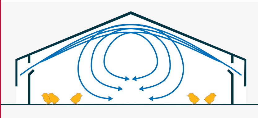
Figure 102 Correct air flow during minimum ventilation.
