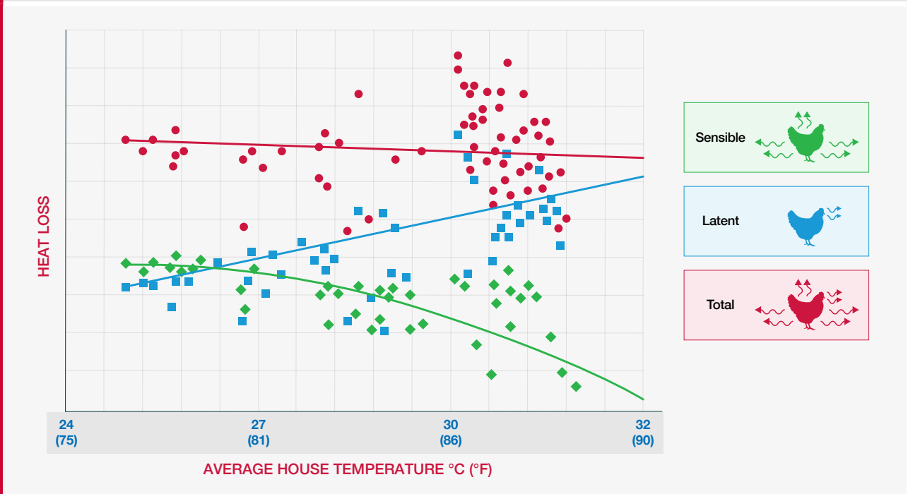
Figure 113 Sensible and latent heat loss.
