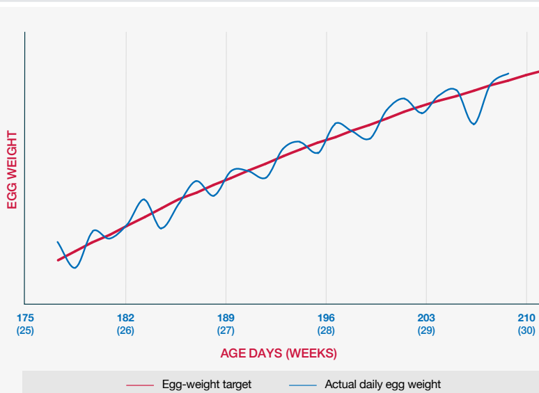
Figure 55 An example showing normal fluctuations in the daily weight of bulk-weighed eggs.
