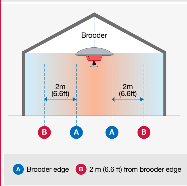
Figure 16 Spot brooding temperature gradients.
