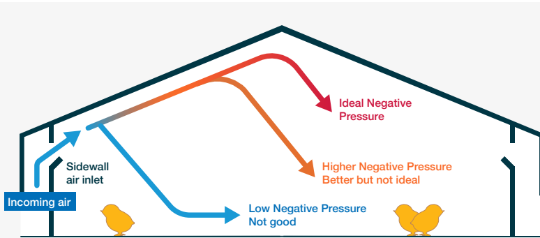
Figure 101 Using negative pressure to control air speed.
