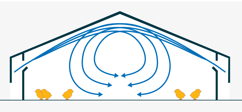
Figure 102 Correct air flow during minimum ventilation.
